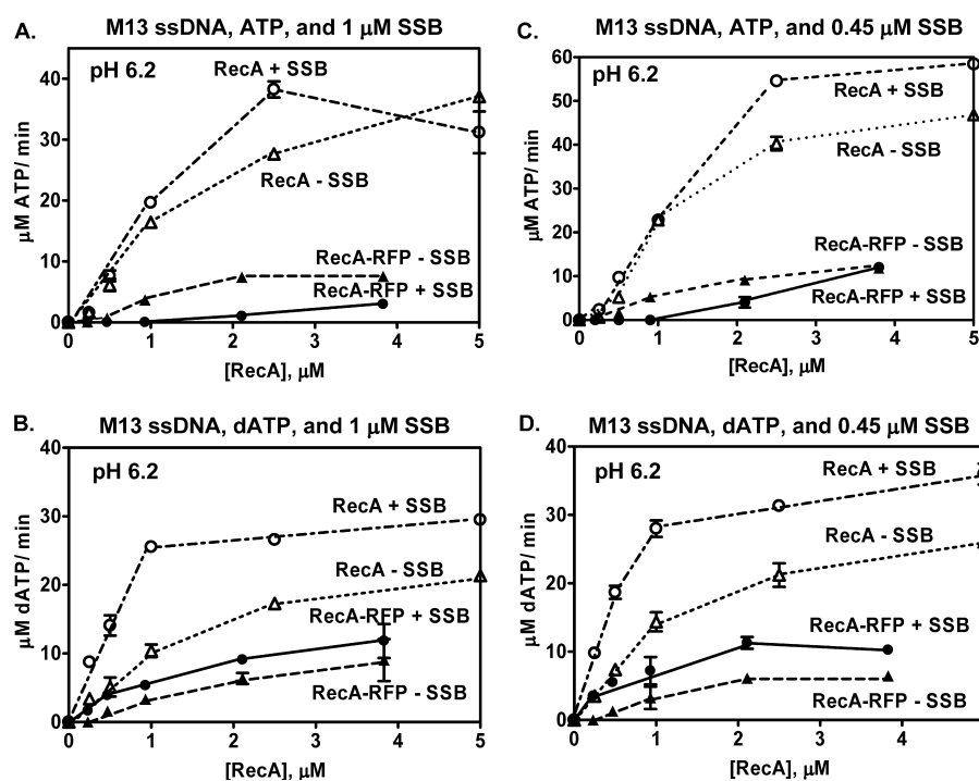
FIGURE 5. The M13 ssDNA-dependent ATP hydrolysis of RecA-RFP protein is not inhibited by SSB protein at pH 6.2. A, M13 ssDNA-dependent ATPase activity in the presence or absence of SSB protein (1 μM). Open triangles, wild-type RecA without SSB; open circles, wild-type RecA with SSB protein; closed triangles, RecA-RFP without SSB protein; closed circles, RecA-RFP with SSB protein. B, M13 ssDNA-dependent dATPase activity in the presence or absence of SSB protein (1 μM). C, M13 ssDNA-dependent ATPase activity in the presence or absence of SSB protein (0.45 μM). D, M13 ssDNA-dependent dATPase activity in the presence or absence of SSB protein (0.45 μM). Symbols in panels B–D are the same as in panel A. Data are mean ± S.D.
